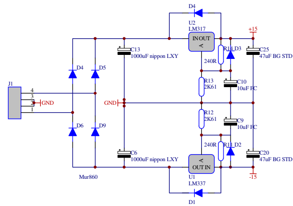
Symetrical voltage regulator Krzysztof Marcinek kafka85@o2.pl
